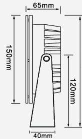
Optional Tripod
